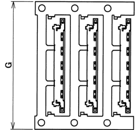
VIEW J (S=2/1)
